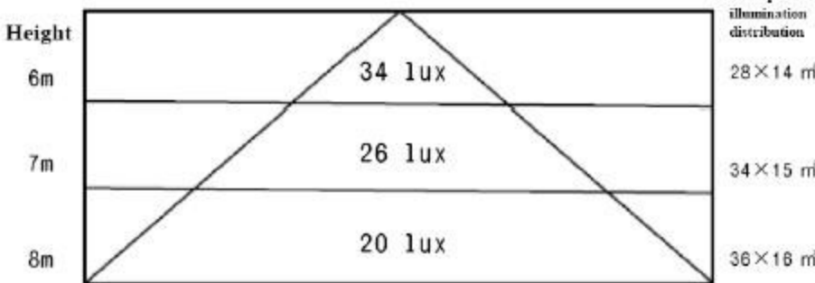
100W LED Street Light's Lux data, height, isotropic illumination distribution
