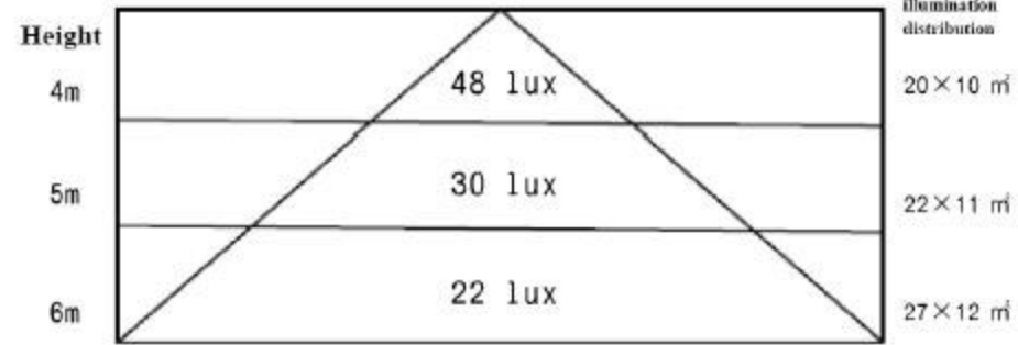
60W LED Street Light's Lux data, height, isotropic illumination distribution
